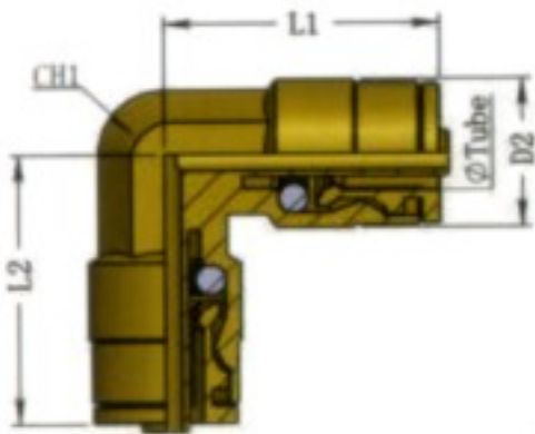
DOT-HUL 等径直角 CR-292
