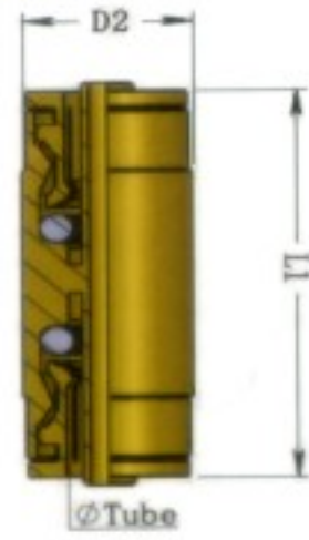
DOT-UC 等径直通 CR-291
